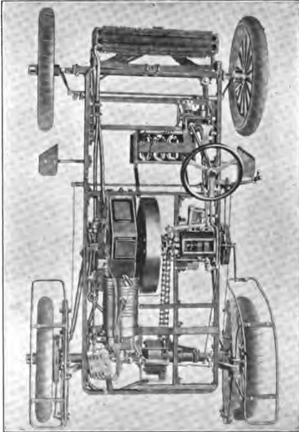
FIG. 405.—Plan of the "Packard" 12 H.P. Tonneau Carriage, showing motor and mechanism in position.
